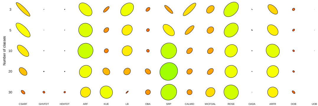
Fig. 38: Comparison of all 15 algorithms on the number of classes under concept drift and multi-class shifting imbalance ratio. Axes of the ellipse represent PMAUC and Kappa metrics. Color gradient represents the product of both metrics.
