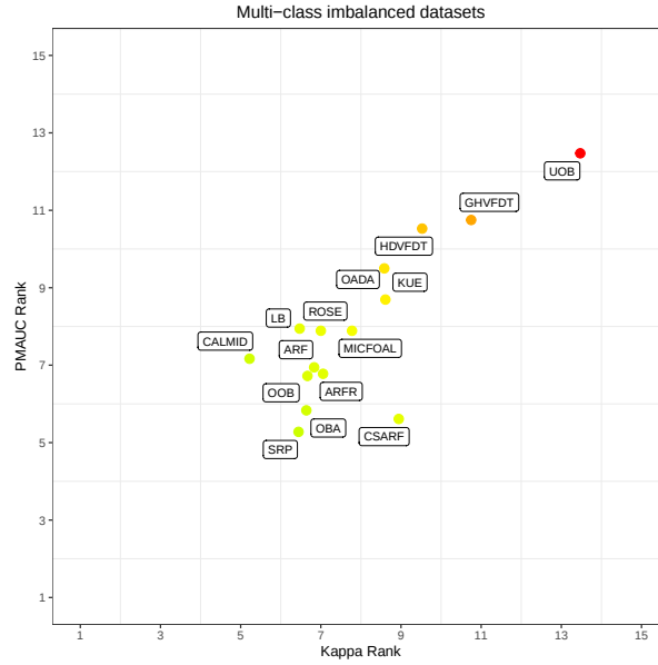
Fig. 40: Comparison of all 15 algorithms for multi-class imbalanced datasets. Color gradient represents the product of both metrics.
