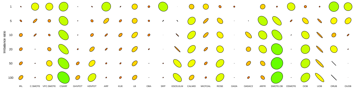
Fig. 17: Comparison of all 24 algorithms for rare instances on static class imbalance ratio. Axes of the ellipse represent G-Mean and Kappa metrics. Color gradient represents the product of both metrics.
