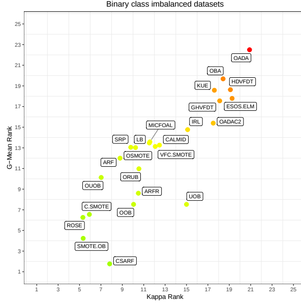
Fig. 28: Comparison of all 24 algorithms for binary class imbalanced datasets. Color gradient represents the product of both metrics.
