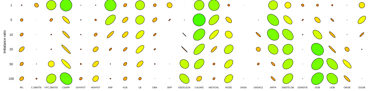
Fig. 19: Comparison of all 24 algorithms for splitting minority clusters on static class imbalance ratio. Axes of the ellipse represent G-Mean and Kappa metrics. Color gradient represents the product of both metrics.
