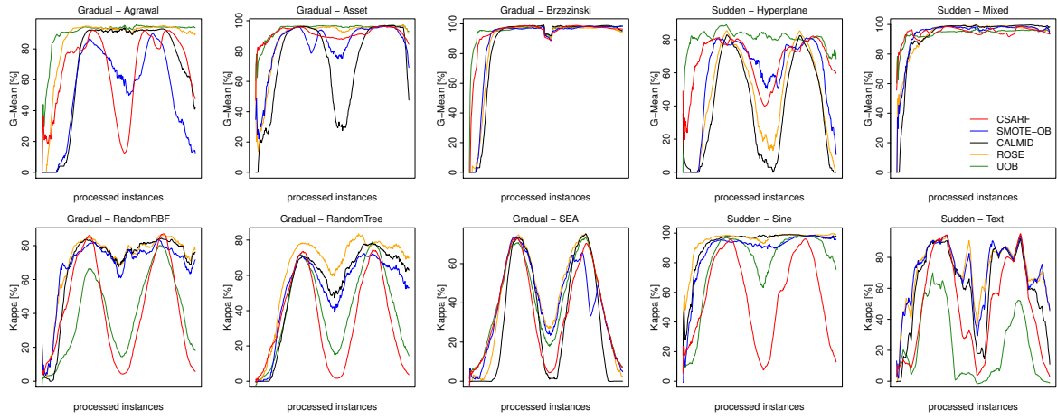
Fig. 9: G-Mean and Kappa on flipping and refliping class imbalance ratio with gradual and sudden drift.
