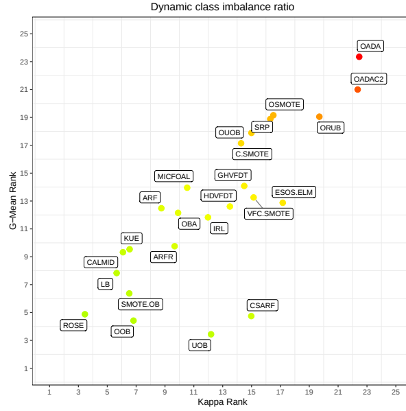
Fig. 10: Comparison of all 24 algorithms for dynamic class imbalance ratio. Color gradient represents the product of both metrics.
