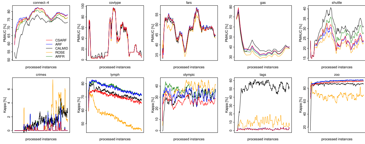
Fig. 39: PMAUC and Kappa on multi-class imbalanced datasets.
