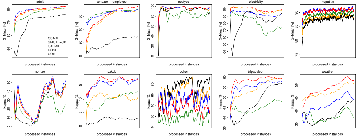
Fig. 27: G-Mean and Kappa on binary class imbalanced datasets.
