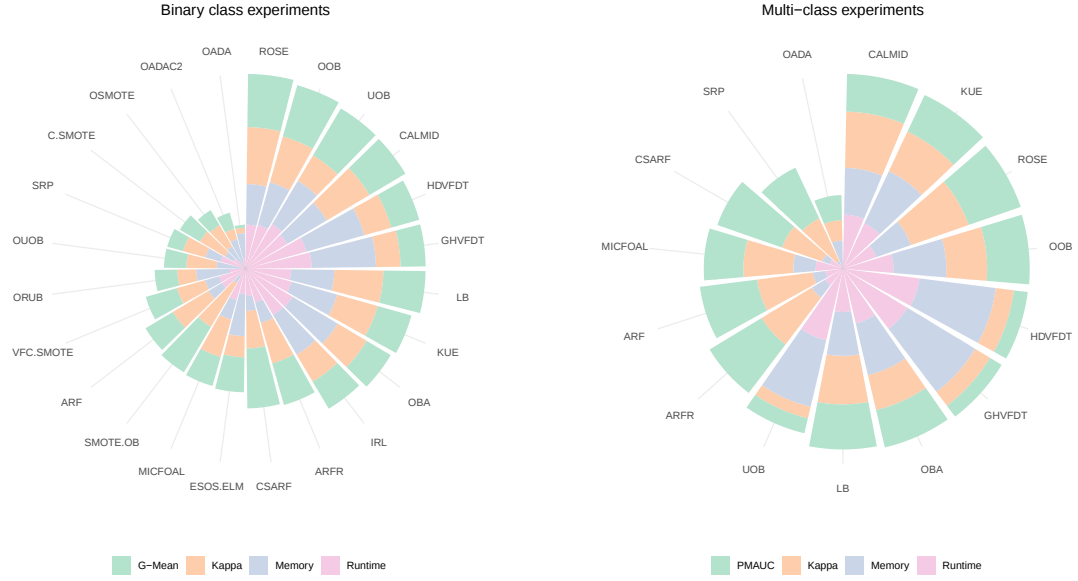
Fig. 45: Overall comparison of stacked algorithms' ranks for G-Mean/PMAUC, Kappa, runtime, and memory on binary and multi-class imbalanced benchmarks. Algorithms are sorted clockwise by the stacked ranks best to worst. Equal weight for the four metrics.
