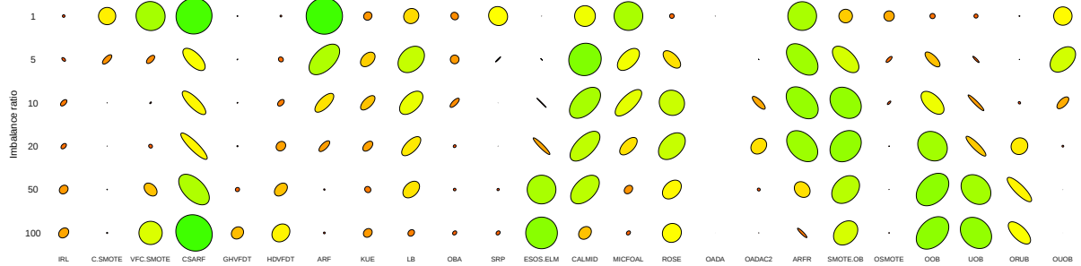
Fig. 20: Comparison of all 24 algorithms for merging minority clusters on static class imbalance ratio. Axes of the ellipse represent G-Mean and Kappa metrics. Color gradient represents the product of both metrics.
