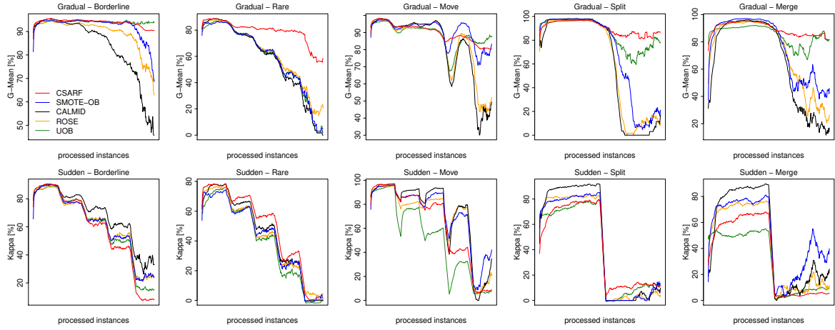
Fig. 21: G-Mean and Kappa on increasing borderline, rare, moving, splitting, and merging minority clusters and increasing imbalance ratio.
