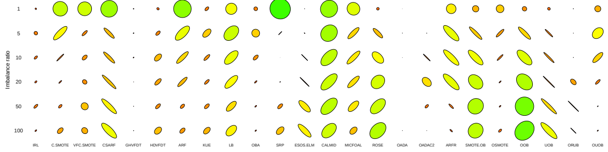
Fig. 16: Comparison of all 24 algorithms for borderline instances on static class imbalance ratio. Axes of the ellipse represent G-Mean and Kappa metrics. Color gradient represents the product of both metrics.
