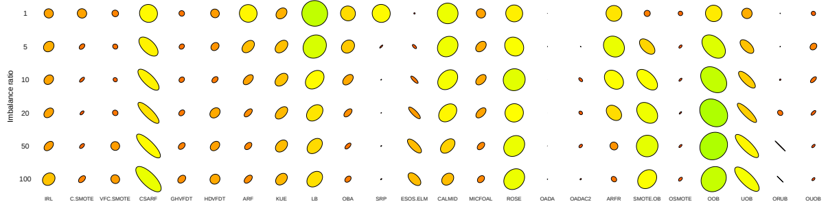
Fig. 5: Comparison of all 24 algorithms for different levels of static class imbalance ratio. The axes of the ellipse represent G-Mean and Kappa metrics. The bigger the axes the better rank of the algorithm on the metrics. The more rounded the ellipse the more agreement between the metrics. The color gradient represents the product of both metrics' ranks.
