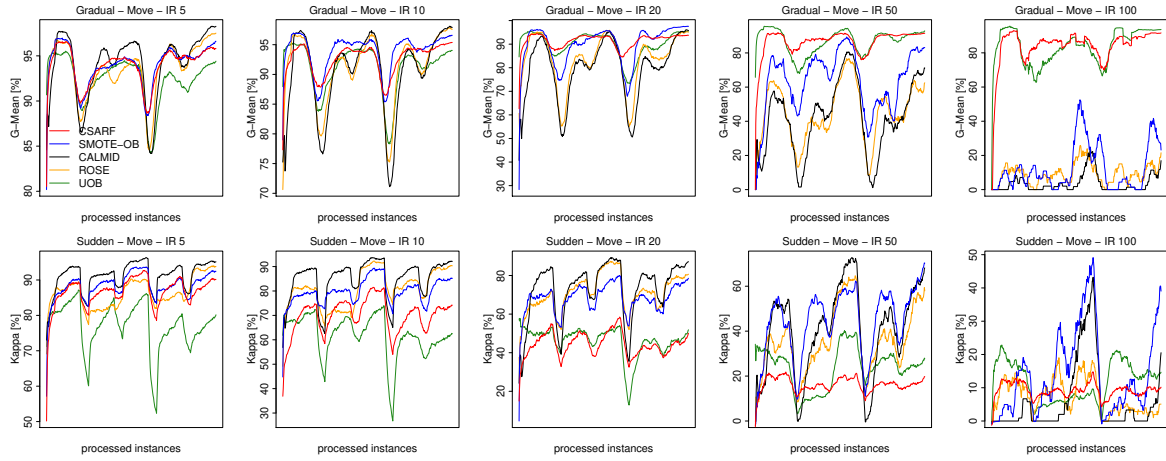
Fig. 13: G-Mean and Kappa on moving minority clusters for static imbalance ratio.
