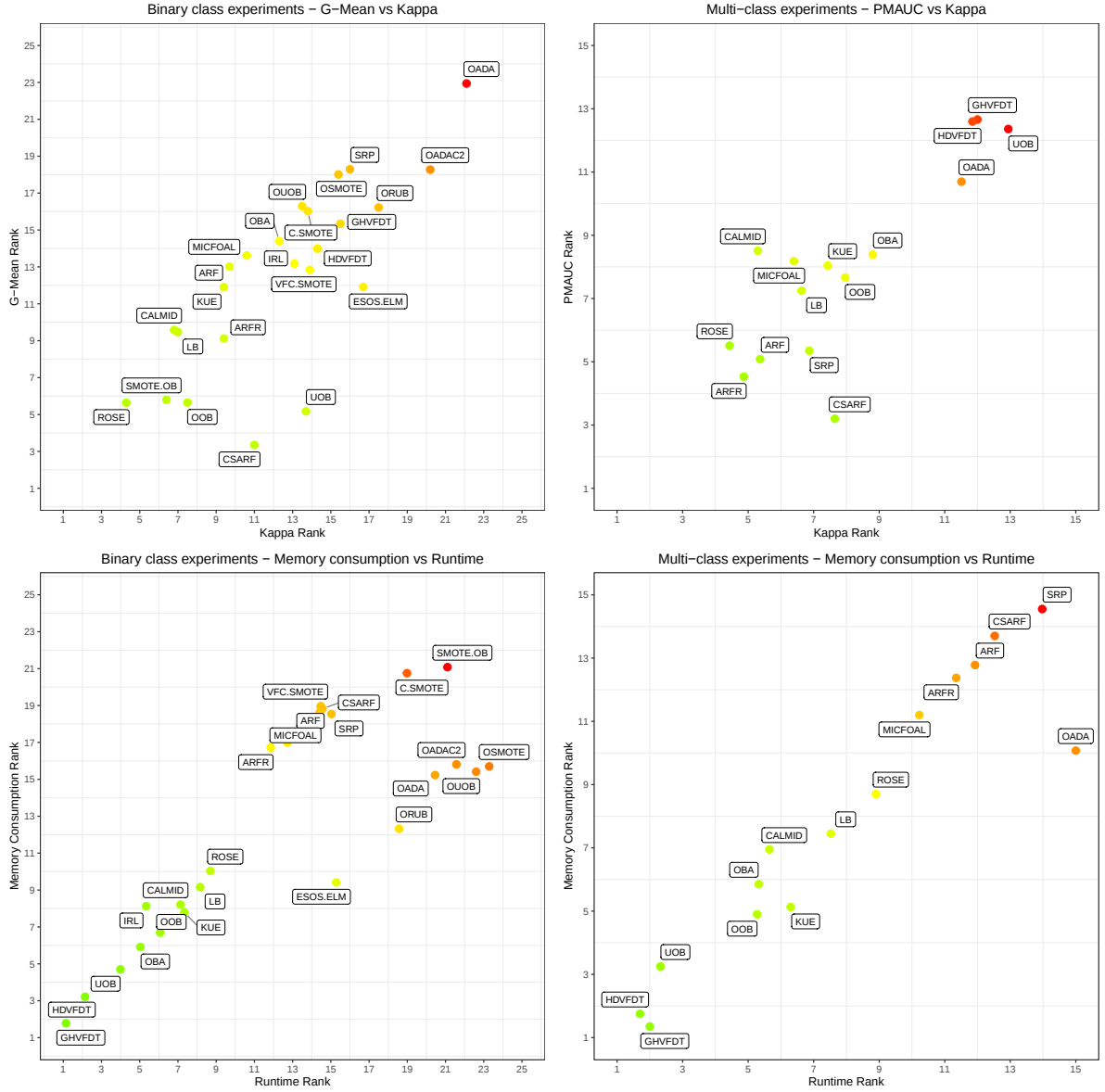
Fig. 43: Overall comparison of algorithms' ranks for G-Mean/PMAUC vs Kappa and Memory Consumption vs Runtime on binary and multi-class imbalanced benchmarks. Color gradient represents the product of each pair of metrics.
