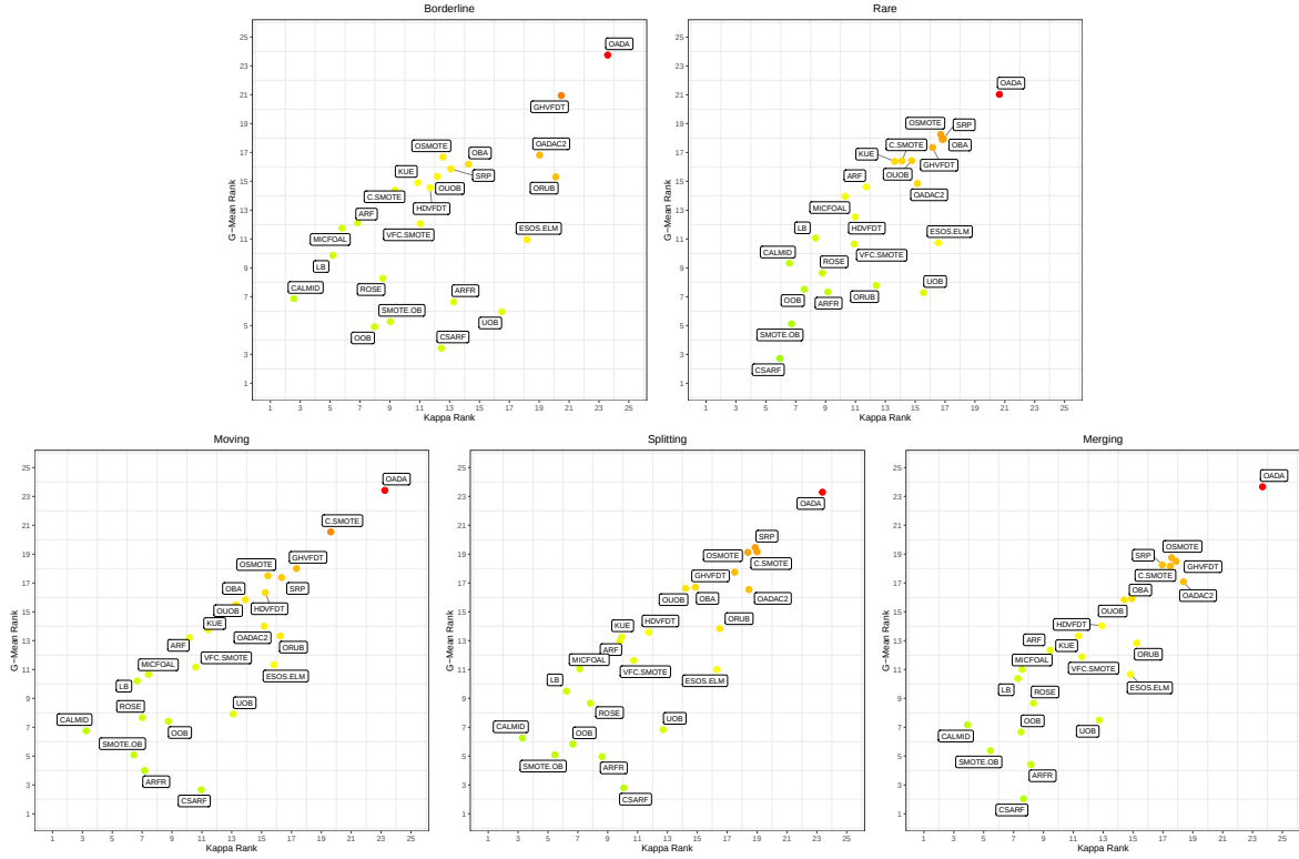
Fig. 22: Comparison of all 24 algorithms on borderline, rare, moving, splitting, merging minority clusters and increasing imbalance ratio. Color gradient represents the product of both metrics.
