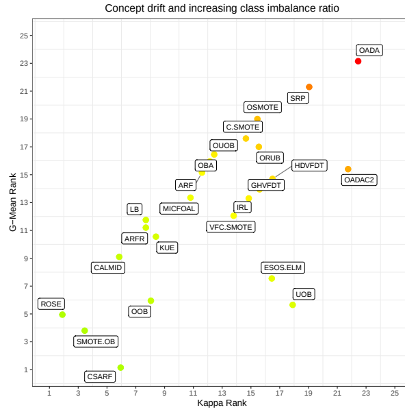
Fig. 26: Comparison of all 24 algorithms for concept drift with increasing class imbalance ratio. Color gradient represents the product of both metrics.
