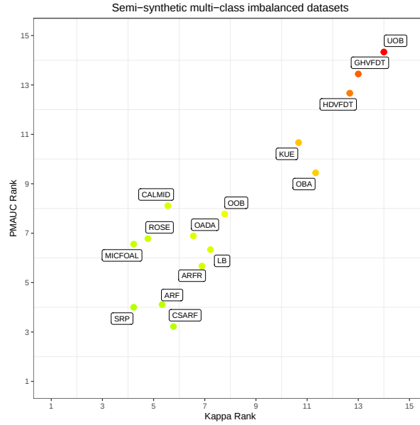
Fig. 42: Comparison of all 15 algorithms for semi-synthetic multi-class imbalanced datasets. Color gradient represents the product of both metrics.
