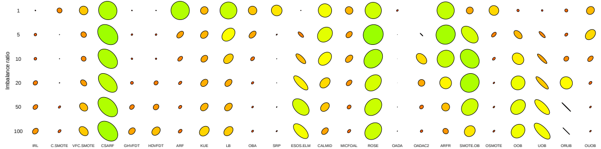
Fig. 24: Comparison of all 24 algorithms for concept drift with static class imbalance ratio. Axes of the ellipse represent G-Mean and Kappa metrics. Color gradient represents the product of both metrics.
