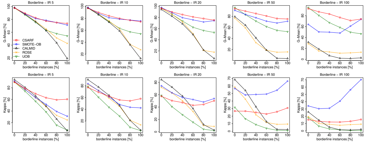
Fig. 11: Robustness to borderline instances for static imbalance ratio (G-Mean and Kappa).
