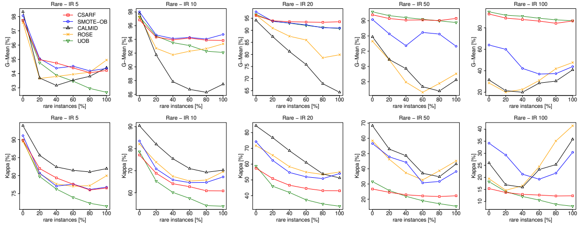
Fig. 12: Robustness to rare instances for static imbalance ratio (G-Mean and Kappa).
