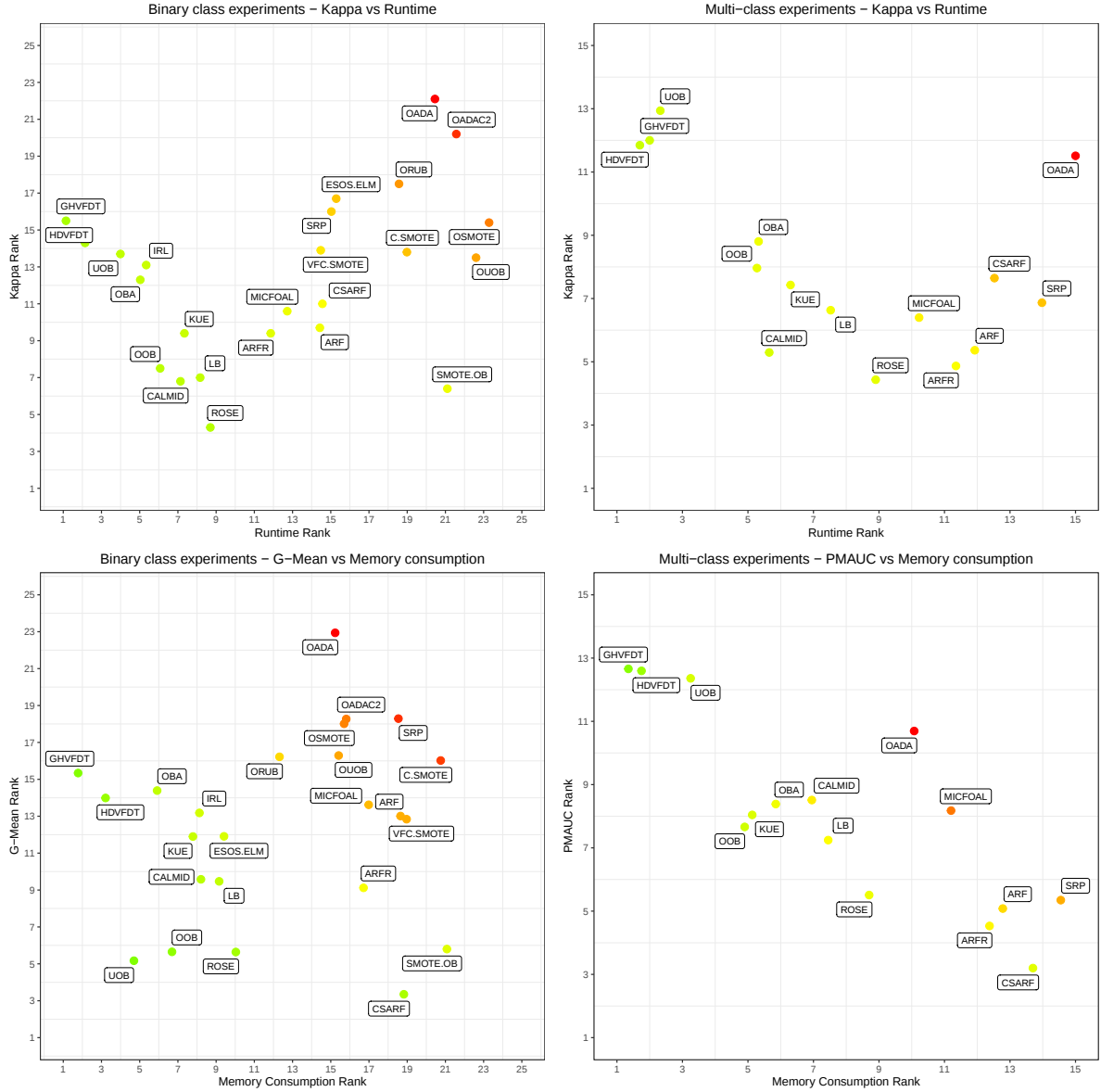
Fig. 44: Overall comparison of algorithms' ranks for G-Mean/PMAUC/Kappa vs Runtime/Memory Consumption on binary and multi-class imbalanced benchmarks. Color gradient represents the product of each pair of metrics.
