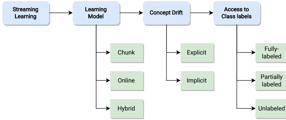
Fig. 1: Streaming learning taxonomy.
