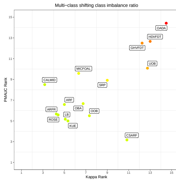
Fig. 32: Comparison of all 15 algorithms for multi-class shifting class imbalance ratio. Color gradient represents the product of both metrics.
