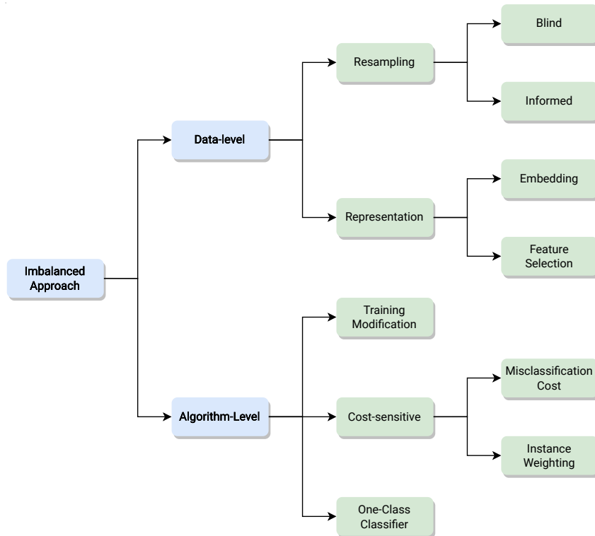
Fig. 2: Taxonomy of approaches for imbalanced data streams.
