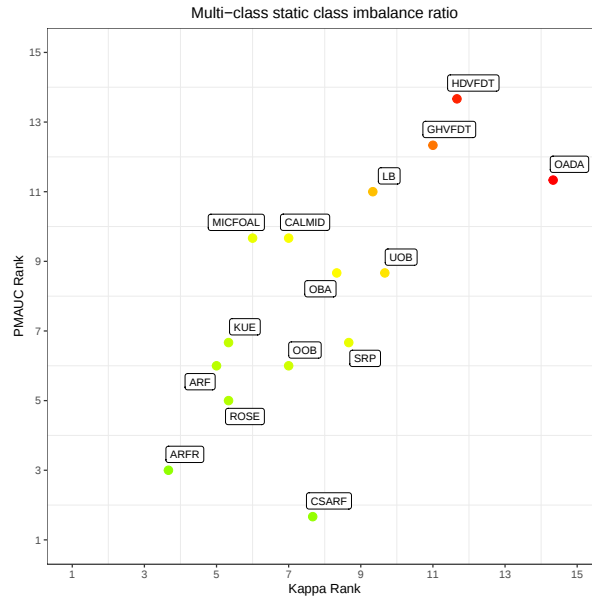
Fig. 30: Comparison of all 15 algorithms for multi-class static class imbalance ratio. Color gradient represents the product of both metrics.
