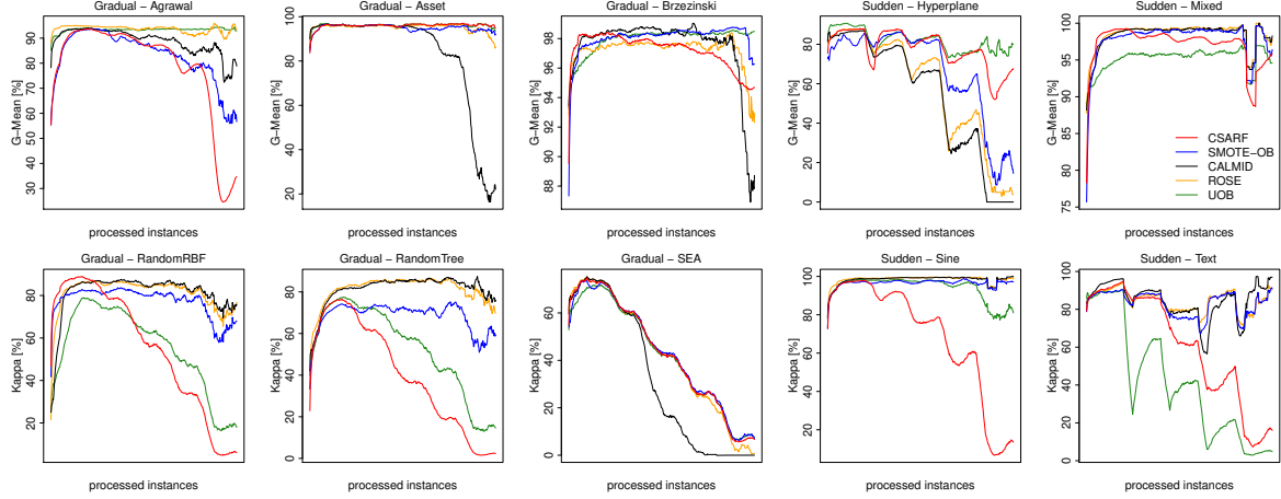
Fig. 6: G-Mean and Kappa on increasing class imbalance ratio with gradual and sudden drift.
