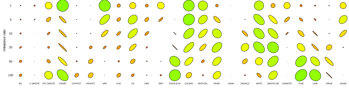
Fig. 18: Comparison of all 24 algorithms for moving minority clusters on static class imbalance ratio. Axes of the ellipse represent G-Mean and Kappa metrics. Color gradient represents the product of both metrics.
