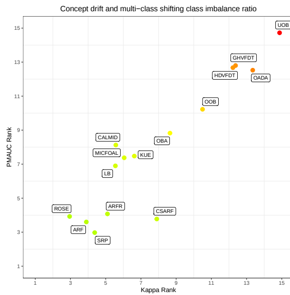
Fig. 36: Comparison of all 15 algorithms on concept drift and multi-class shifting class imbalance ratio. Color gradient represents the product of both metrics.
